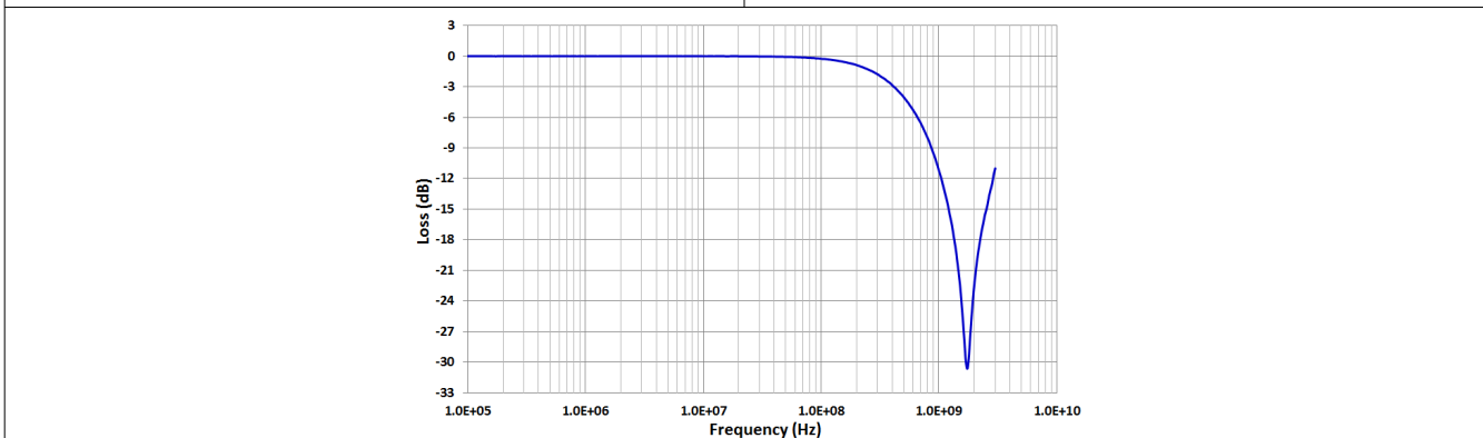
Figure 6-9. Insertion Loss
