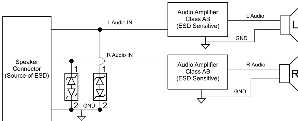
Figure 8-1. Typical Application Schematic
