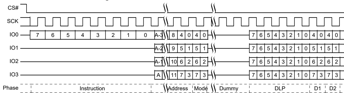
Figure 74. DDR Quad I/O Read Initial Access
