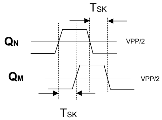
Output-Output Skew
