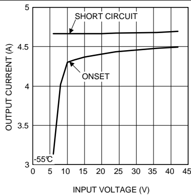
Figure 27. Current Limit 3.3 V OUT at -55°C
