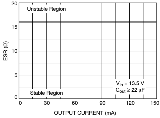
Figure 17. ESR Stability vs. Output Current (3.3 V Version)
