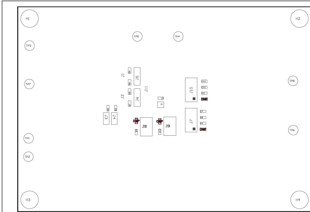
Figure 2-2. Component Placement - Top Overlay
