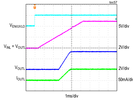
MAX17671F, 3.3V LINEAR REGULATOR START-UP FROM ENUVULO FIGURE 6 CIRCUIT
