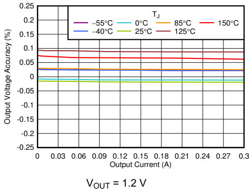
Figure 6-1. Output Accuracy vs I_{OUT}
