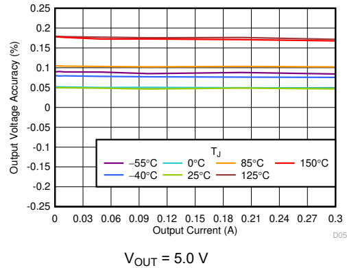
Figure 6-2. Output Accuracy vs I_{OUT}
