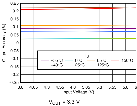
Figure 6-3. Output Accuracy vs V_{IN}
