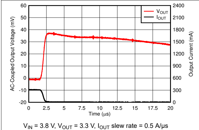
Figure 6-23. I_{OUT} Transient From 1-mA to 300-mA Falling Edge
