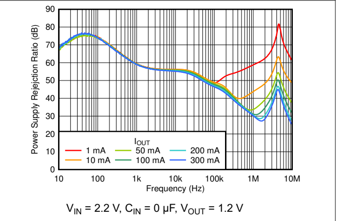
Figure 6-24. PSRR vs Frequency and I_{OUT}
