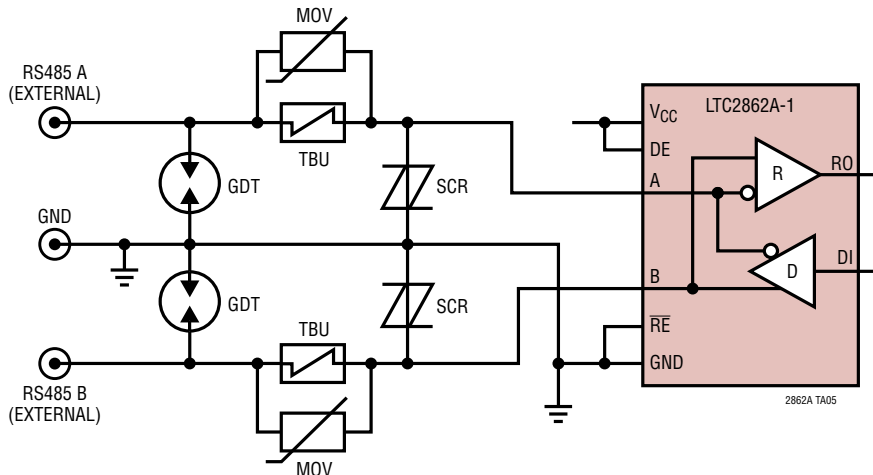
Network for IEC Level 4 Protection Against 5kV Surge, 5kV EFT and 30kV IEC ESD Plus \pm 360V Overvoltage Protection
