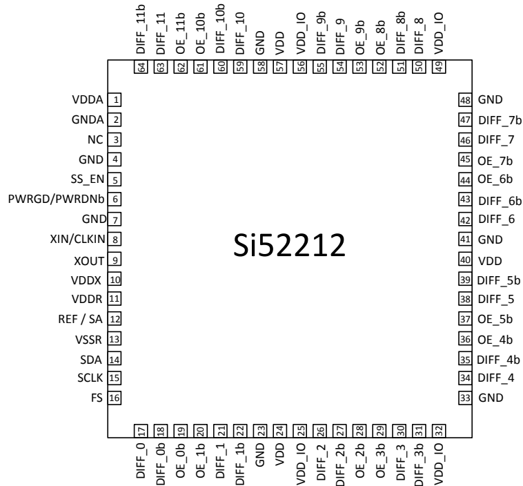
Figure 9.1. 64-Pin QFN
