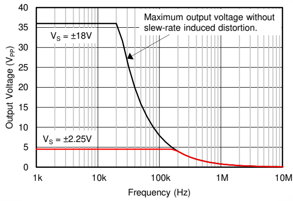
Figure 6-37. Maximum Output Voltage Amplitude vs Frequency
