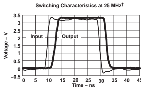
† AUP1G08 data at C_L = 15 pF
