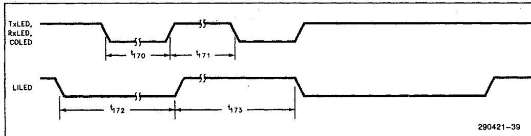
Figure 40. LED Timings
