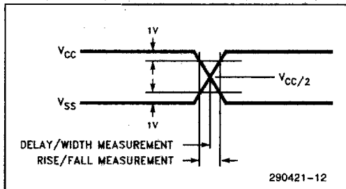
Figure 13. Voltage Levels for TDH, TDL, \overline{\text{TDH}} , and \overline{\text{TDL}} .
