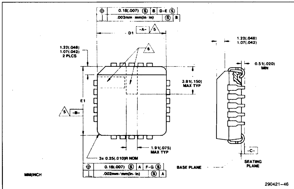
Figure 46. Molded Details
