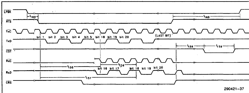
Figure 38. Loopback Timings
