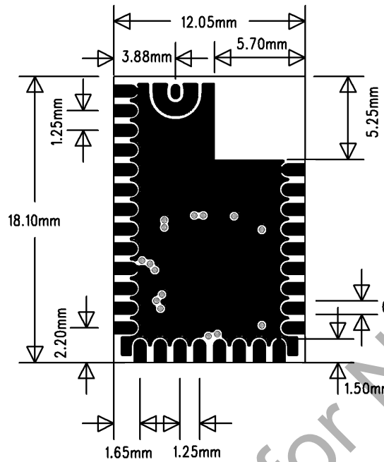
Figure 8: Physical dimensions and pinout (top view)
