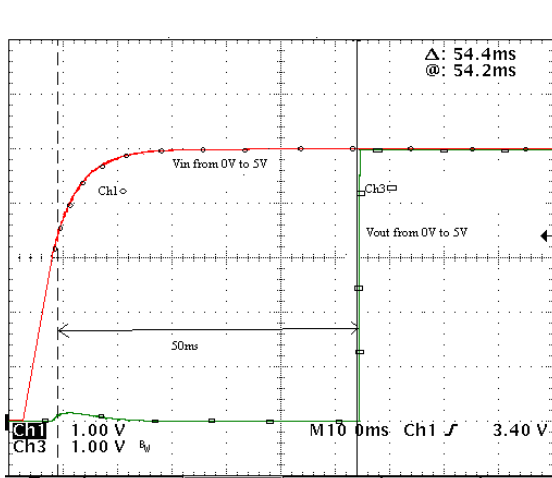
Figure 7. Startup V_{in} = Ch1, V_{out} = Ch3
