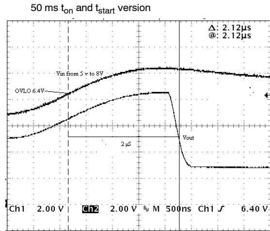
Figure 8. Output Turn Off Time V_{in} = Ch1, V_{out} = Ch2
