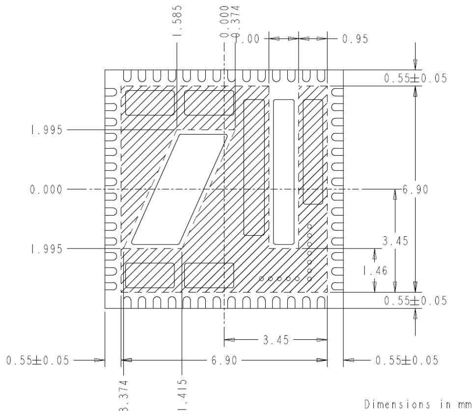
Figure 9: Lead-Frame exposed metal (Bottom View)
