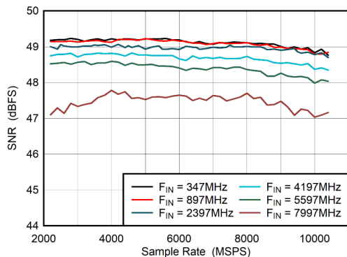
Figure 6-29. DES Mode: SNR vs Sample Rate
