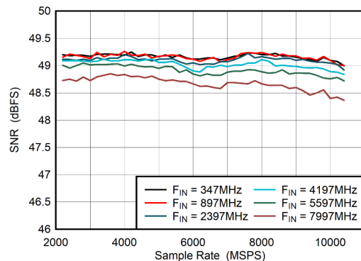
Figure 6-30. DES Mode: SNR vs Sample Rate
