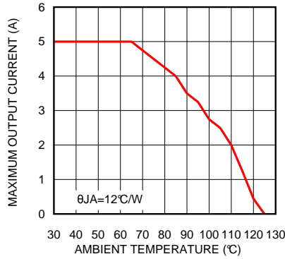
V_{IN} = 12\text{ V} , V_{OUT} = 5\text{ V}
