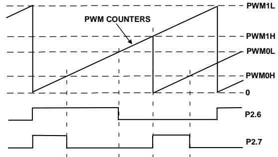
Figure 61. PWM Mode 5
