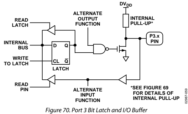
Figure 70. Port 3 Bit Latch and I/O Buffer
