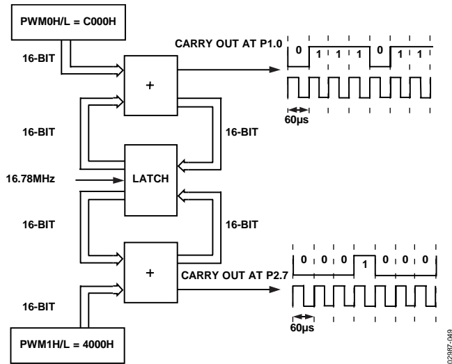
Figure 60. PWM Mode 4
