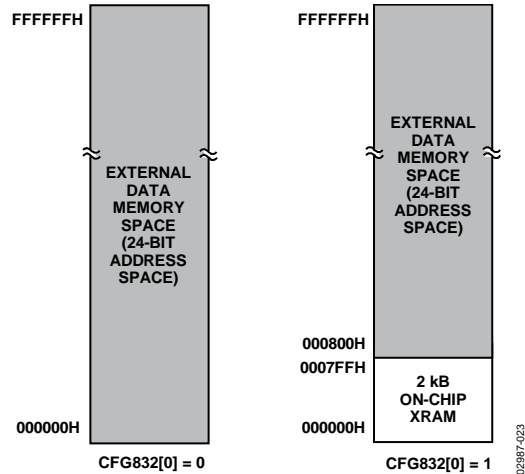
Figure 34. Internal and External XRAM
