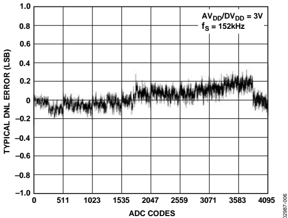
Figure 17. Typical DNL Error, V_{DD} = 3V
