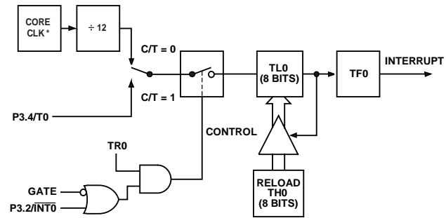
Figure 77. Timer/Counter 0, Mode 2
