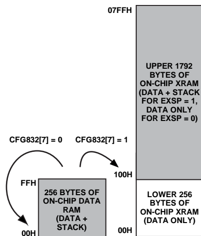
Figure 33. Extended Stack Pointer Operation
