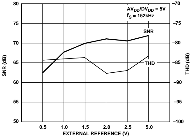
Figure 28. Typical Dynamic Performance vs. V_{REF} , V_{DD} = 5\text{ V}
