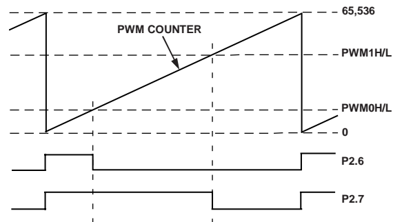
Figure 59. PWM Mode 3
