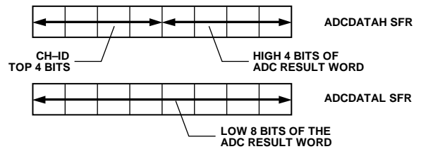
Figure 38. ADC Result Format
