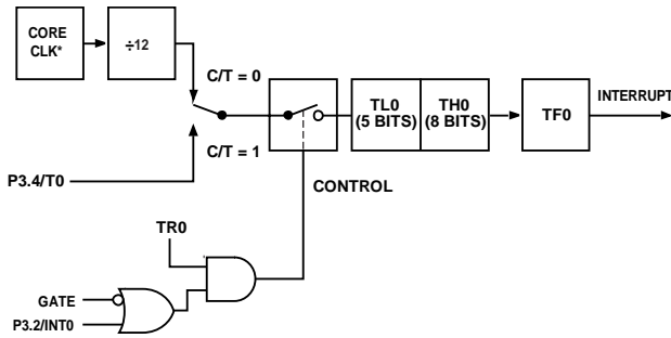
Figure 75. Timer/Counter 0, Mode 0
