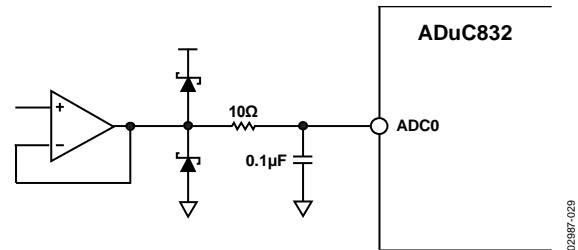
Figure 40. Buffering Analog Inputs
