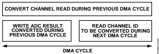
Figure 46. DMA Cycle
