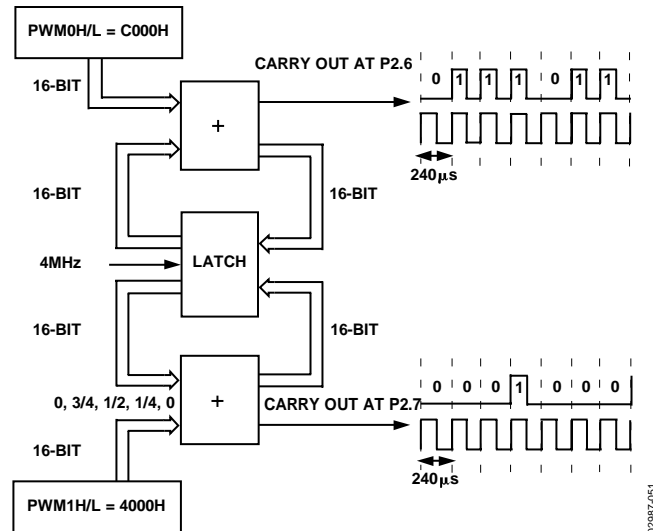
Figure 62. PWM Mode 6
