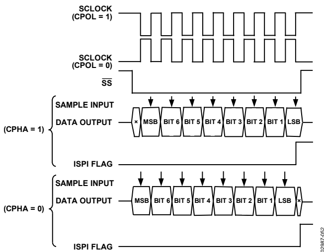
Figure 63. SPI Timing, All Modes
