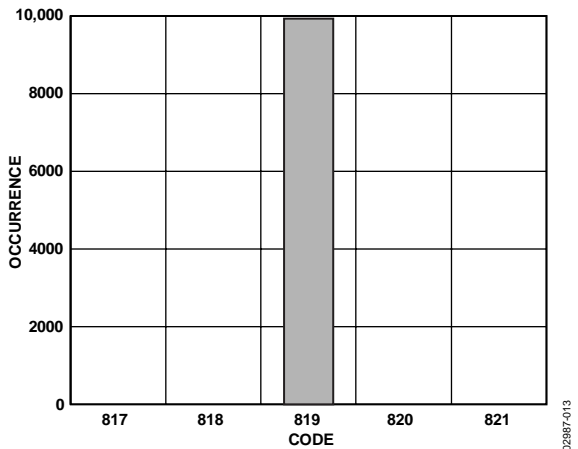
Figure 24. Code Histogram Plot, V_{DD} = 5V
