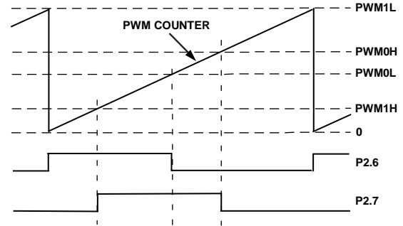
Figure 58. PWM Mode 2
