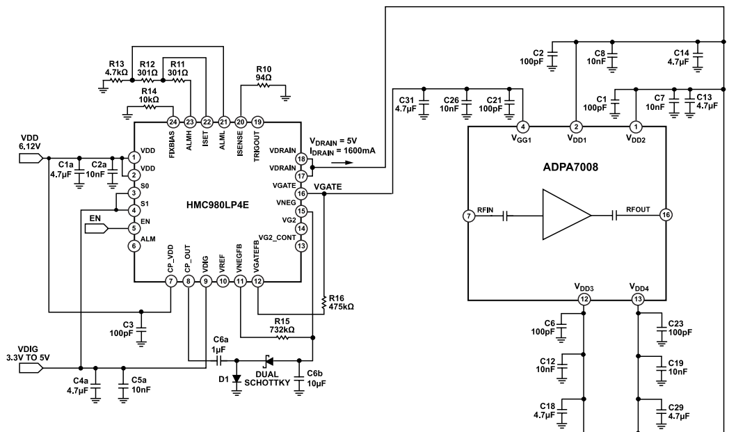
Figure 75. Application Circuit Using HMC980LP4E with ADPA7008 (Internal Negative Voltage Source)
