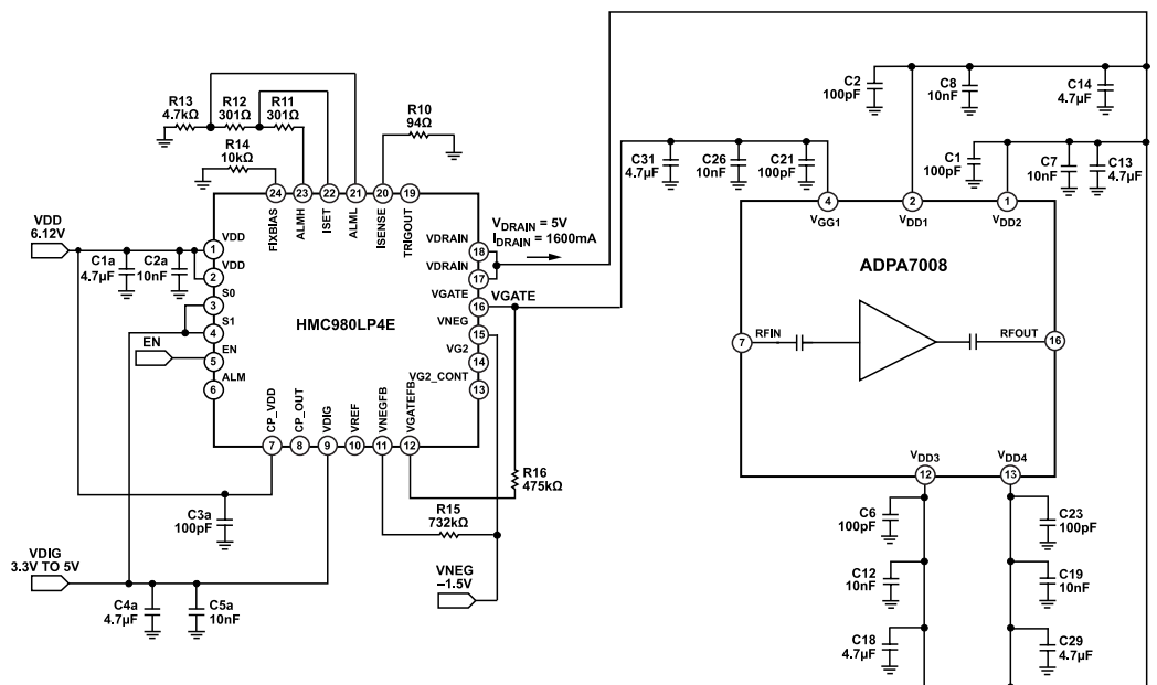
Figure 76. Application Circuit Using HMC980LP4E with ADPA7008 (External Negative Voltage Source)
