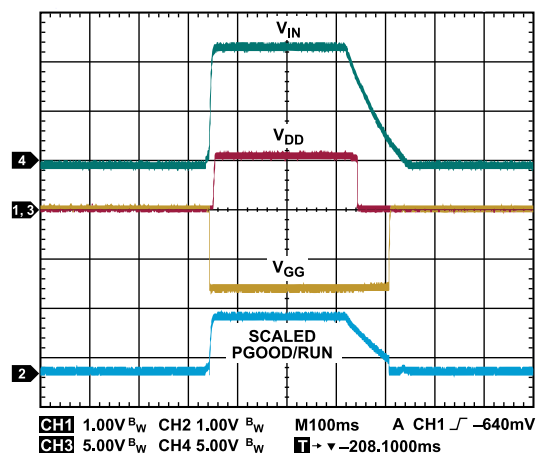
Figure 73. Turn On Sequence and Turn Off Sequence
