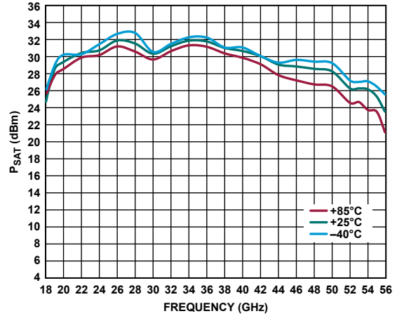
Figure 25. P_{SAT} vs. Frequency for Various Temperatures, V_{DD} = 5\text{ V} , I_{DQ} = 1500\text{ mA}
