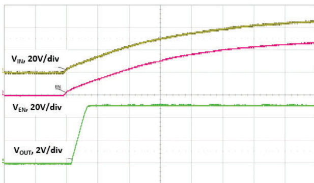
Fig. 30 - Start-up with V_{IN} , Time = 5 ms/div
