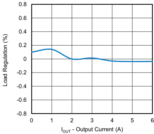
Fig. 22 - Load Regulation
