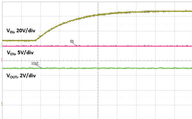
Fig. 29 - Line Transient (8 V to 48 V), Time = 10 ms/div
