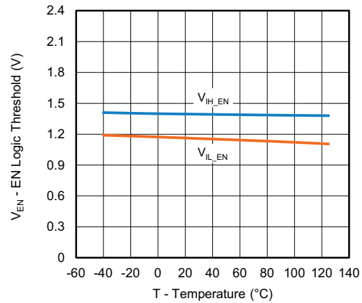
Fig. 25 - EN Logic Threshold vs. Junction Temperature
