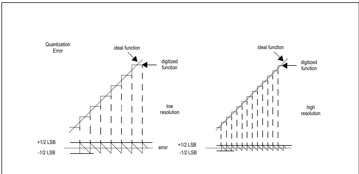
Figure 40: Quantization Error of a Low Resolution and a High Resolution System
