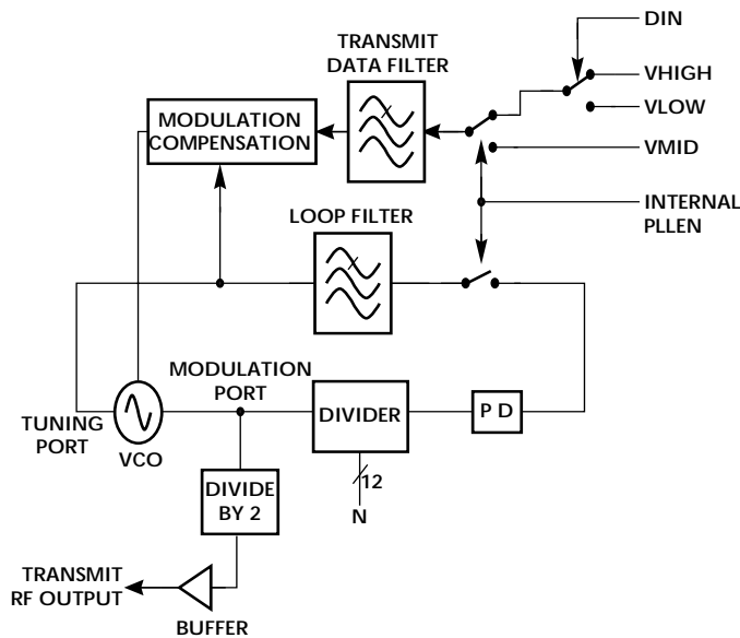
Figure 4. Transmitter Block Diagram
