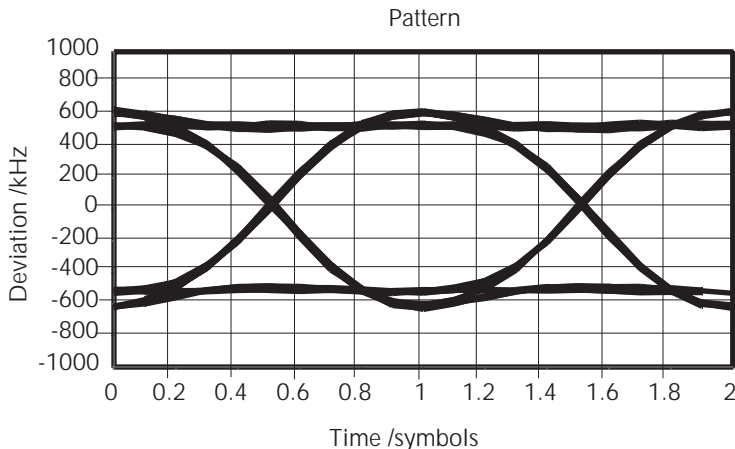
Figure 7. Transmitter Eye Diagram
