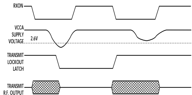
Figure 8. Transmitter Low Voltage Lockout Sequence
