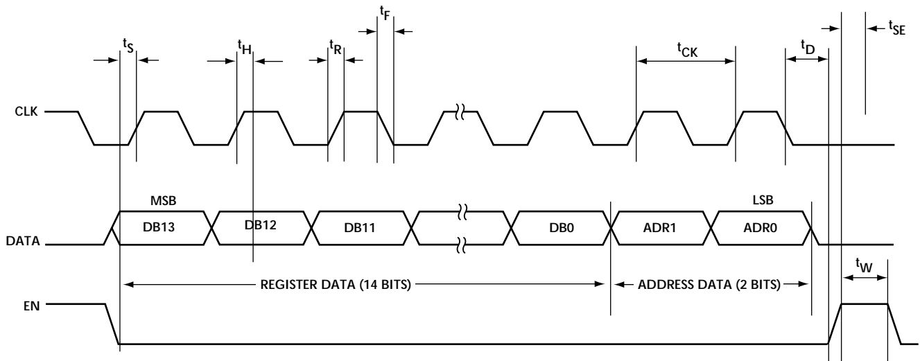
Figure 11. Serial Bus Timing for Address and Data Programming
