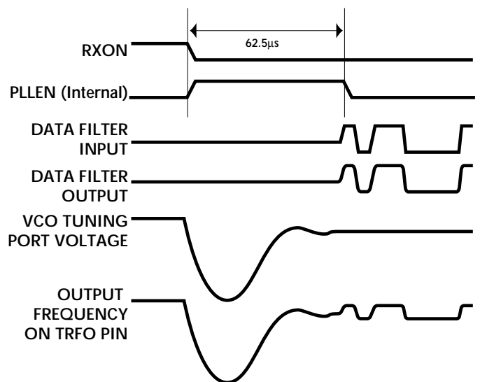
Figure 5. Transmitter Operating Cycle
