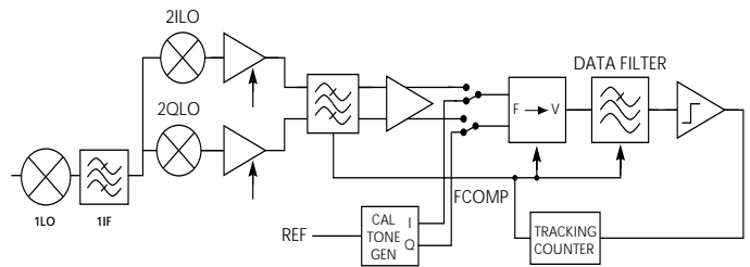
Figure 3. Filter Alignment
