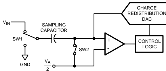
Figure 3. ADC121S101 in Track Mode
