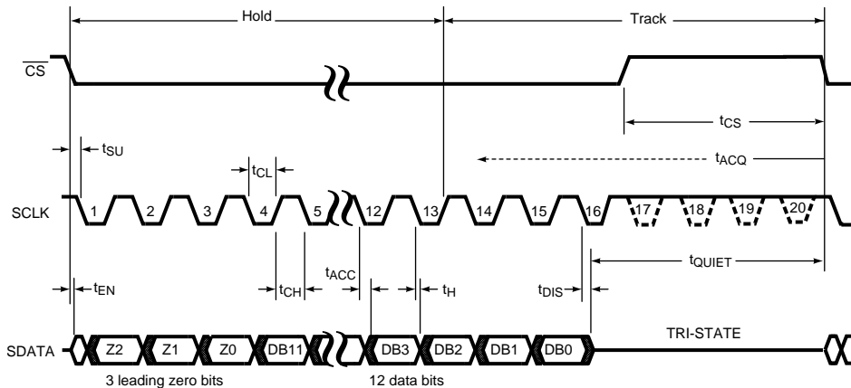
Figure 2. ADC121S101 Serial Timing Diagram
