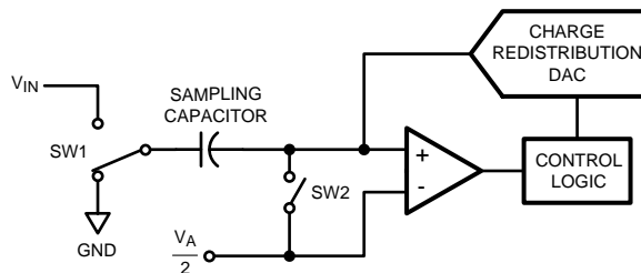
Figure 4. ADC121S101 in Hold Mode
