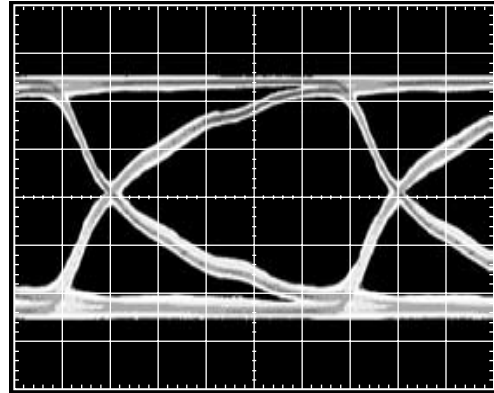
Figure 18. Eye Pattern; 1.244 Gbps, V CC = 3.3 V, PRBS 31 V CC = 3.3V V IN = 2V p-p 38.7mV/DIV 133.7ps/DIV 20dB ATTENUATION TA = 25°C
