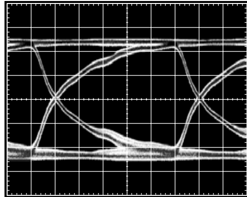
Figure 19. Eye Pattern; 1 Gbps, V CC = 2.5 V, PRBS 31 V CC = 2.5V V IN = 1V p-p 20mV/DIV 166.3ps/DIV 20dB ATTENUATION TA = 25°C
