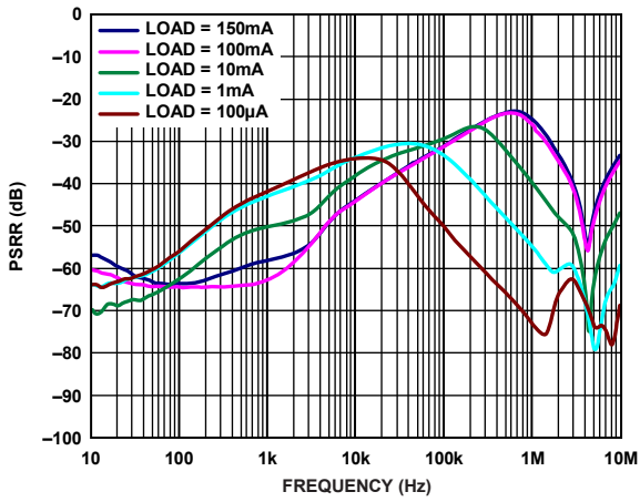
Figure 19. Power Supply Rejection Ratio vs. Frequency, V_{OUT} = 3.3\text{ V} , V_{IN} = 4.3\text{ V}
