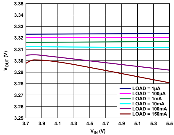
Figure 9. Output Voltage ( V_{OUT} ) vs. Input Voltage ( V_{IN} )
