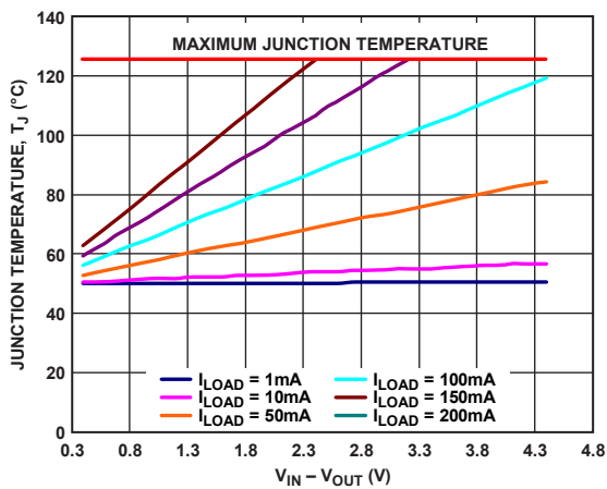
Figure 44. 100 mm 2 of PCB Copper, WLCSP, T_A = 50^\circ\text{C}
