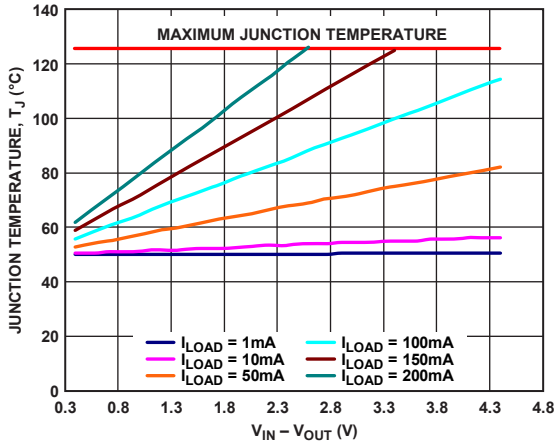
Figure 48. 100 mm 2 of PCB Copper, T_{SO1} , T_A = 50^\circ\text{C}
