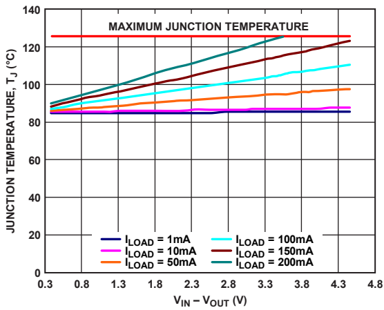
Figure 49. WLCSF, T_A = 85^\circ\text{C}
