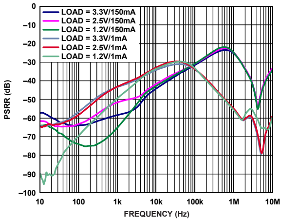
Figure 20. Power Supply Rejection Ratio vs. Frequency Various Output Voltages and Load Currents, V_{IN} - V_{OUT} = 1\text{ V}
