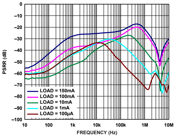
Figure 21. Power Supply Rejection Ratio vs. Frequency Various Output Voltages and Load Currents, V_{OUT} = 2.5\text{ V} , V_{IN} = 3.0\text{ V}
