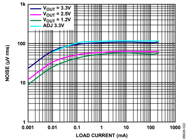
Figure 24. Output Noise vs. Load Current and Output Voltage, V_{IN} = 5\text{ V} , C_{OUT} = 1\text{ }\mu\text{F}
