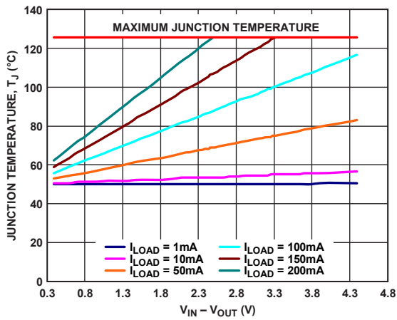
Figure 43. 500 mm 2 of PCB Copper, WLCSP, T_A = 85^\circ\text{C}
