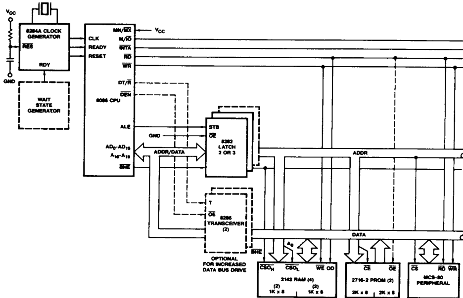
Figure 2a. Minimum Mode 8086 Typical Configuration
