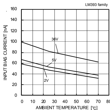
Input Bias Current - Ambient Temperature
