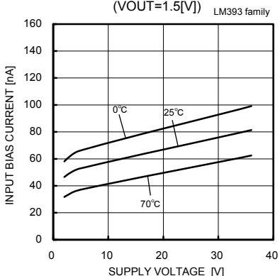
Input Bias Current - Supply Voltage
