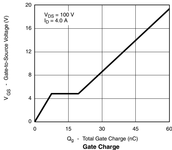
Gate Charge vs. Gate-to-Source Voltage
