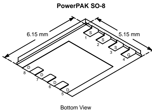
Bottom View Ordering Information: Si7840DP-T1
